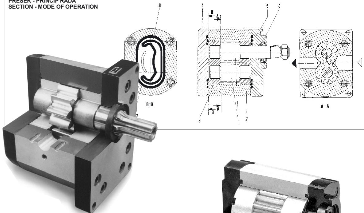
PRESEK - PRINCIP RADA SECTION - MODE OF OPERATION
